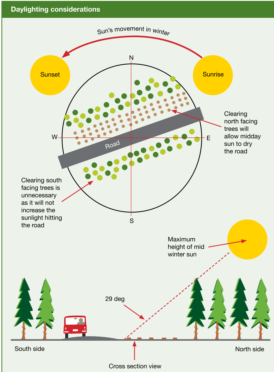
5.5 – Position of mid-winter sun and the effect of cutting north-facing trees for daylighting
